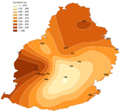
TOTAL MONTHLY SUNSHINE HOURS FOR JUNE 2026
