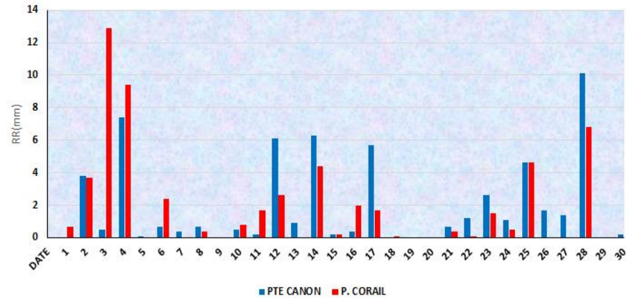
RAINFALL OVER RODRIGUES FOR THE MONTH OF JUNE 2026
