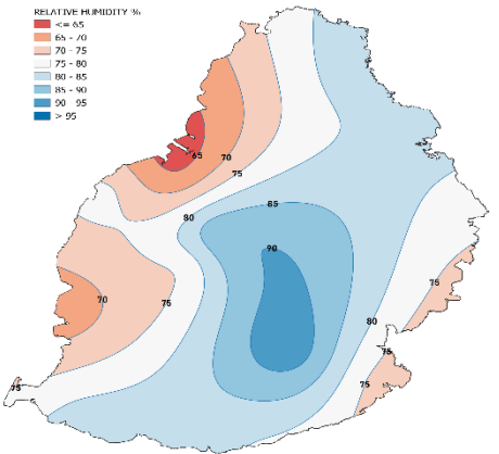
MEAN MONTHLY RELATIVE HUMIDITY (%) FOR JUNE 2026
