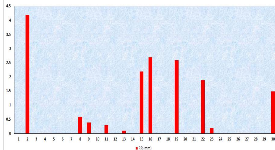
AGALEGA-RAINFALL FOR JUNE 2026
